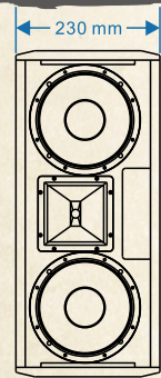
结构图纸 Construction Drawing:
