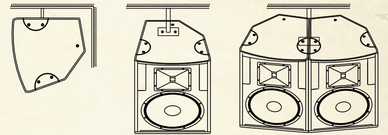
固定安装 Application and installation
